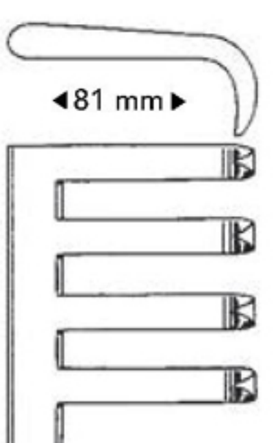
GR771.13 14 cm/5½"
